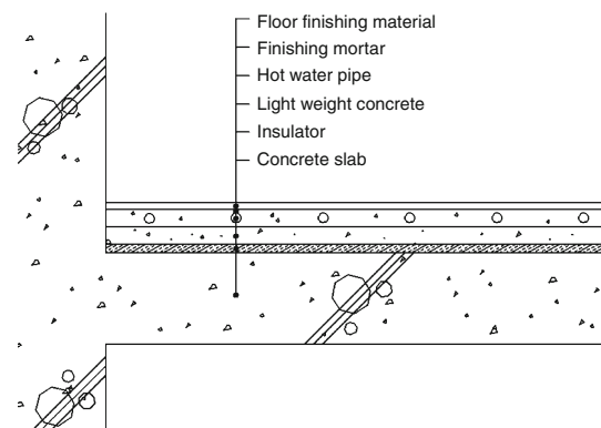
Fig. 3 Standard floor formation for the Korean Ministry of Land
