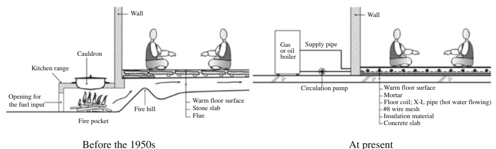
Fig. 1 The radiant floor heating system [57]
