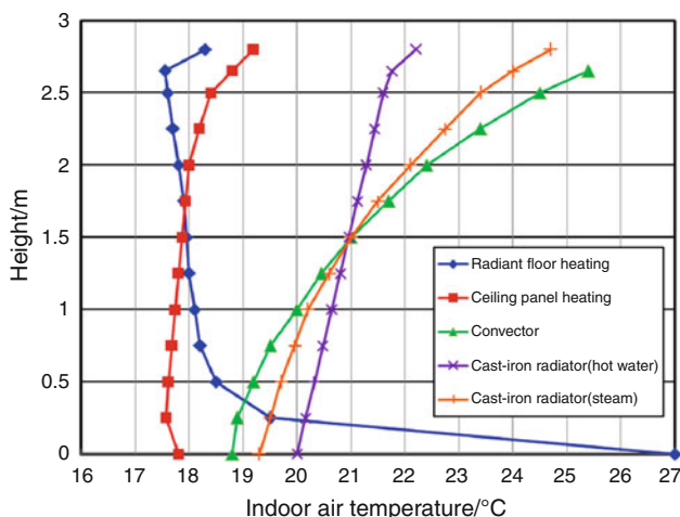
Fig. 2 Comparison of indoor temperature distribution on heating systems
